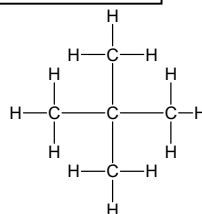
2,2-dimethylpropane
