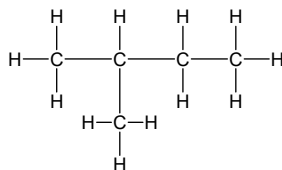
2-methylbutane
