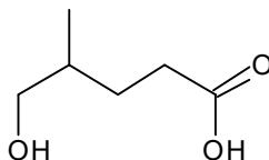
5-hydroxy-4-methylpentanoic acid
