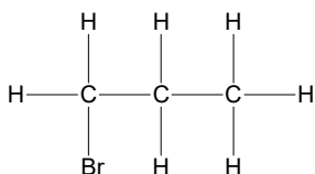
1-bromopropane
