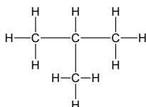
methylpropane
