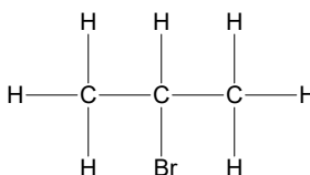
1-bromopropane
