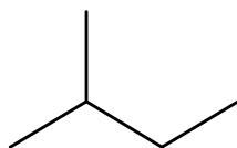
2-methylbutane
